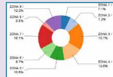
Data Warehouse
