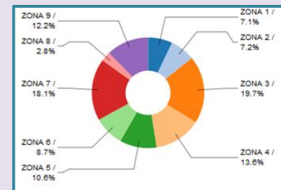
Data Warehouse
